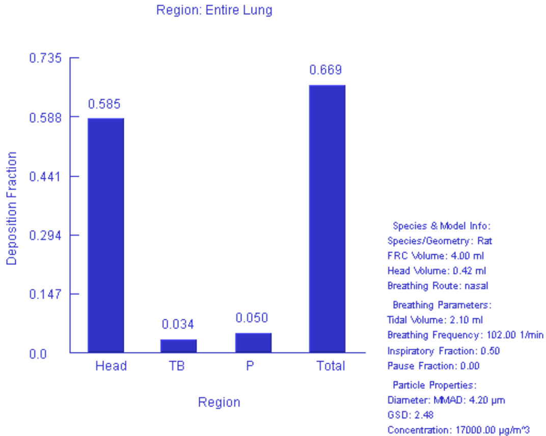
Figure C- 2. MPPD Model Output for Rat (Derelanko et al. 1999)
