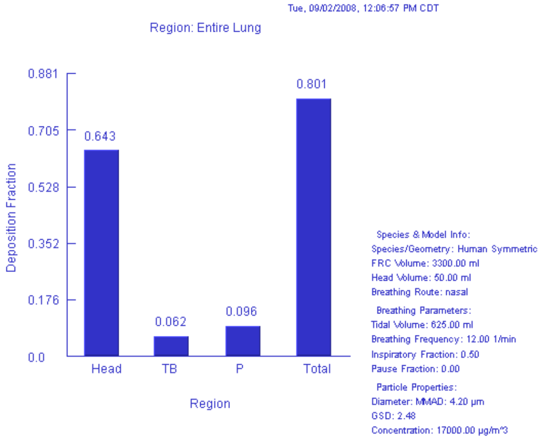
4 5 6 Figure C- 1. MPPD Model Output for Human (Derelanko et al. 1999)
