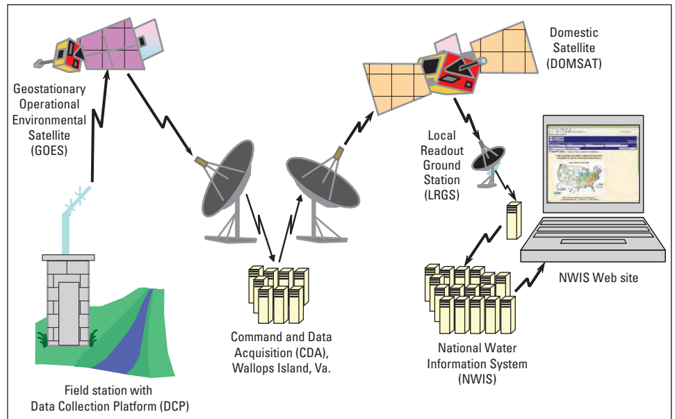
Figure 14. Satellite telemetry is used to transmit near real-time data from streamgages to the USGS National Water Information System for processing (from Nielsen and Norris, 2007).
